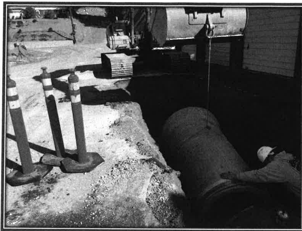
Installation of Drainage Pipe for Tiger Creek Remedy Protection Project Mullan
