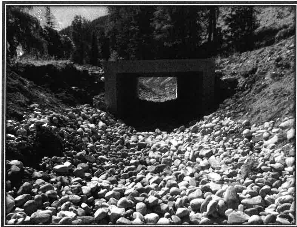
Installation of Fish Passage Structure Rosebud Creek Remedy Protection Project Osburn
