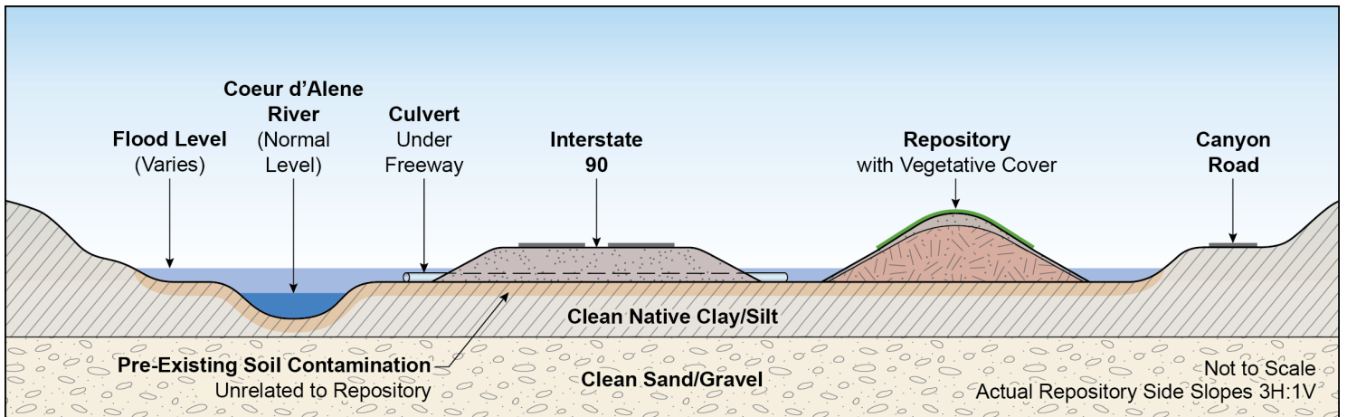
FIGURE 4. High and Low Water Levels at East Mission Flats Repository
