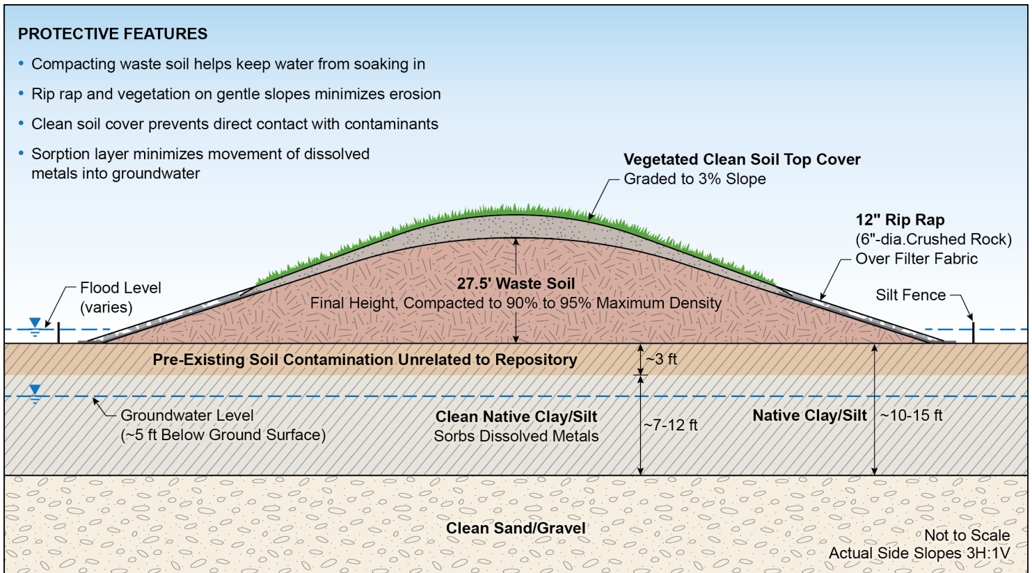
FIGURE 3. Protective Features of East Mission Flats Repository
